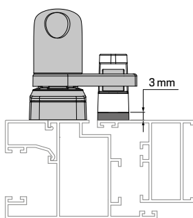
APERTURA EXTERIOR OUTWARD OPENING
